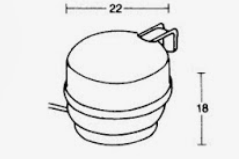
⑨ Egg boiler
