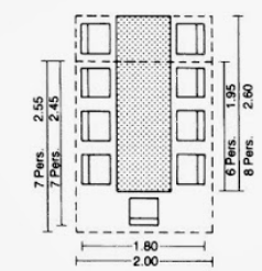
⑱ Minimum area requirements
